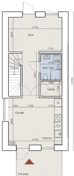
Stueplan Standard
