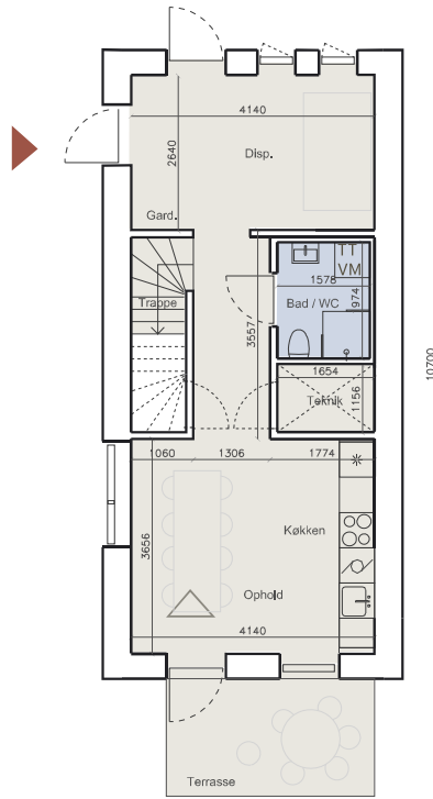
Stueplan Standard
