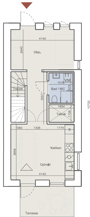
Stueplan Standard
