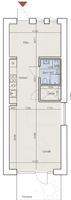
Stueplan Standard
