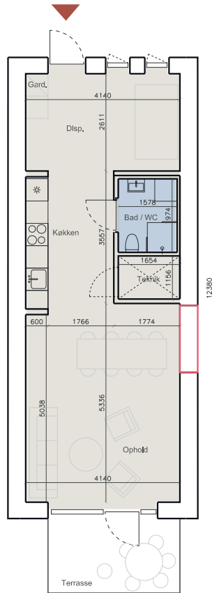
Stueplan Standard
