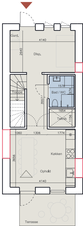
Stueplan Standard
