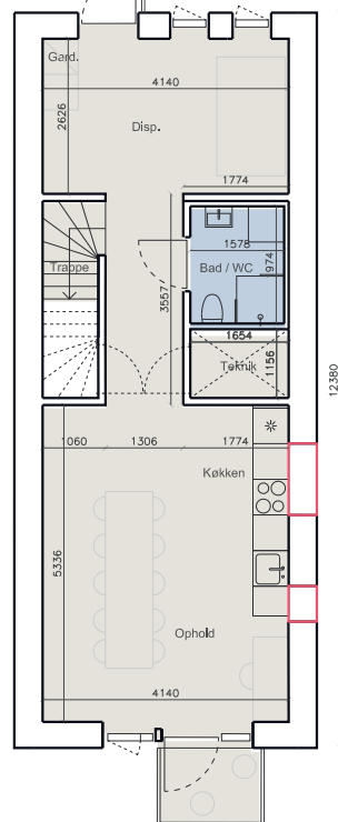
Stueplan Standard
